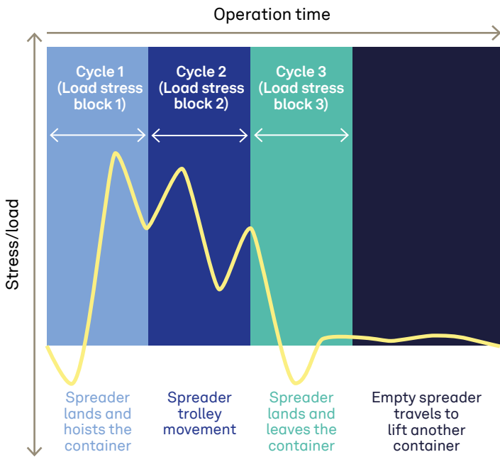
Figure 2. Working cycle definition
