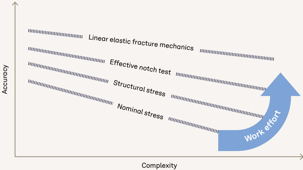
Figure 3. Fatigue strength design methodologies
