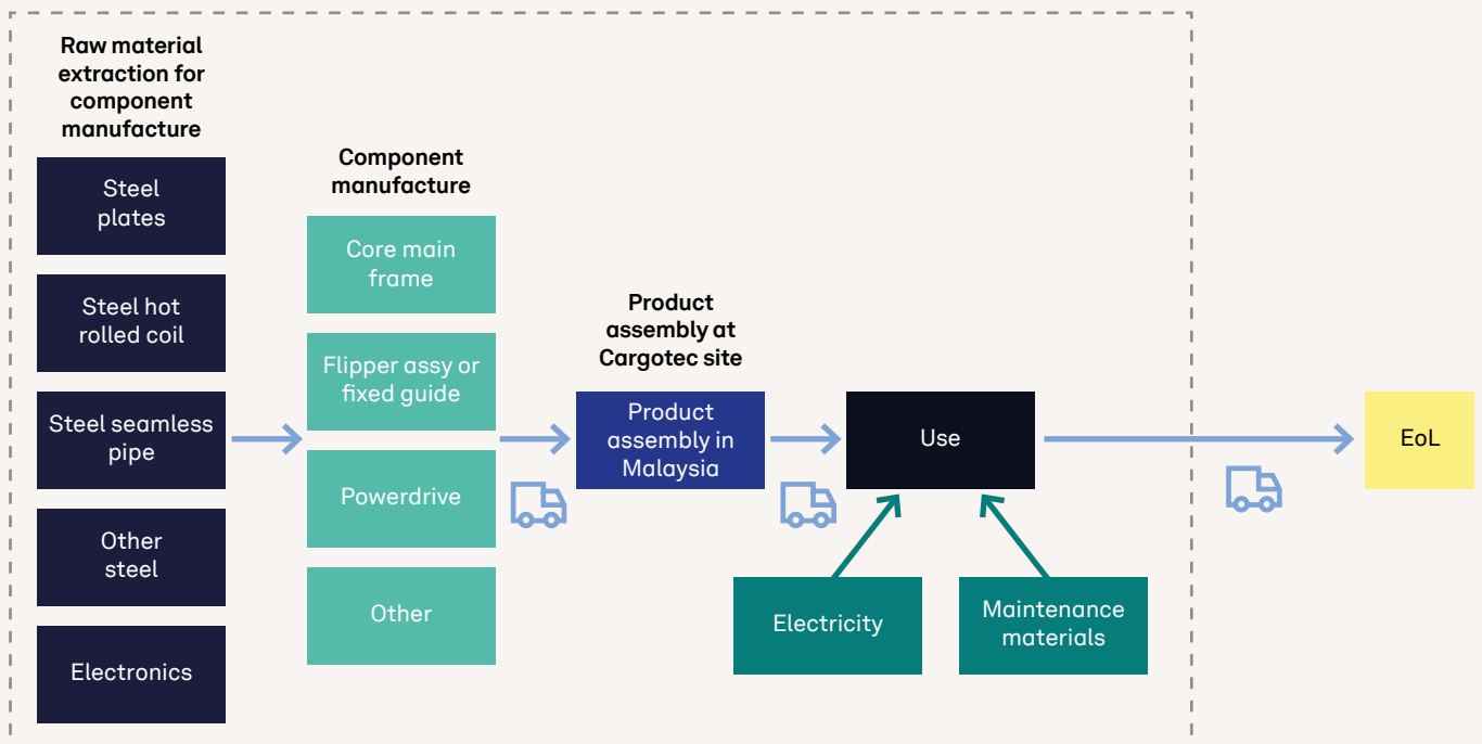
Figure 2. System boundry STS45E
